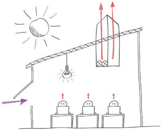
SUMMER STRATEGY Upwards Displacement Ventilation
