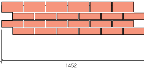
Soffit view
