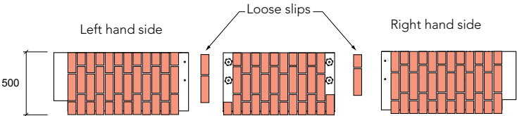
Soffit view
