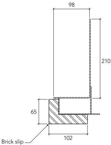
Section view
