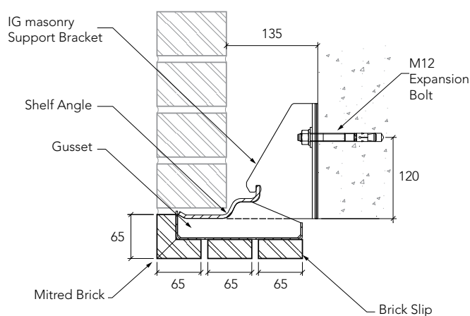
Section view
