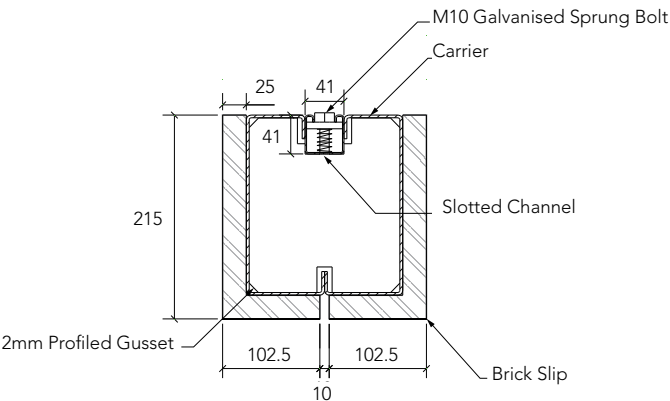
Section view
