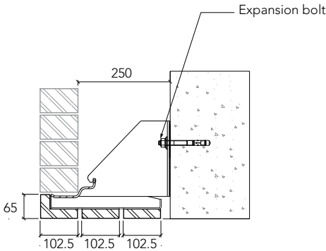
Section view
