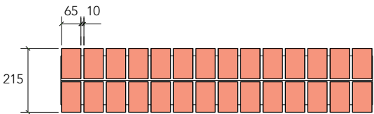
Soffit view
