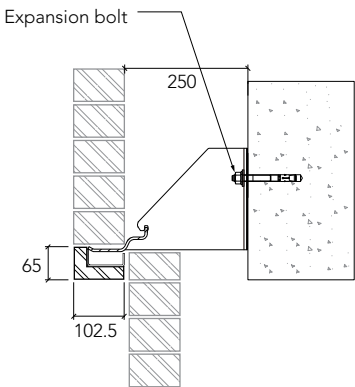
102.5mm SOFFIT
