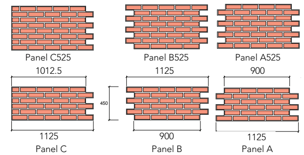
8 No. panel designs
