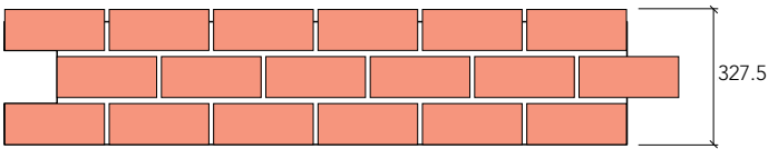
Soffit view
