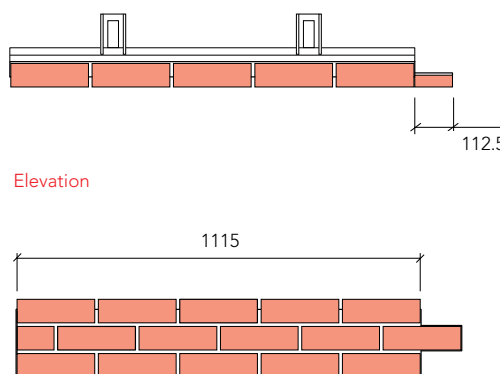
Soffit view
